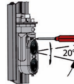
ADJUSTMENT ANGLES VERTICAL 20°
