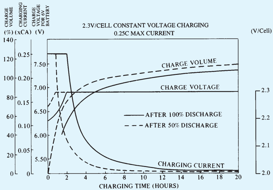
Figure 11. CHARGING CHARACTERISTICS
