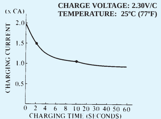
Figure 22. CONSTANT-VOLTAGE CHARGE CHARACTERISTICS WITH NO CURRENT LIMIT
