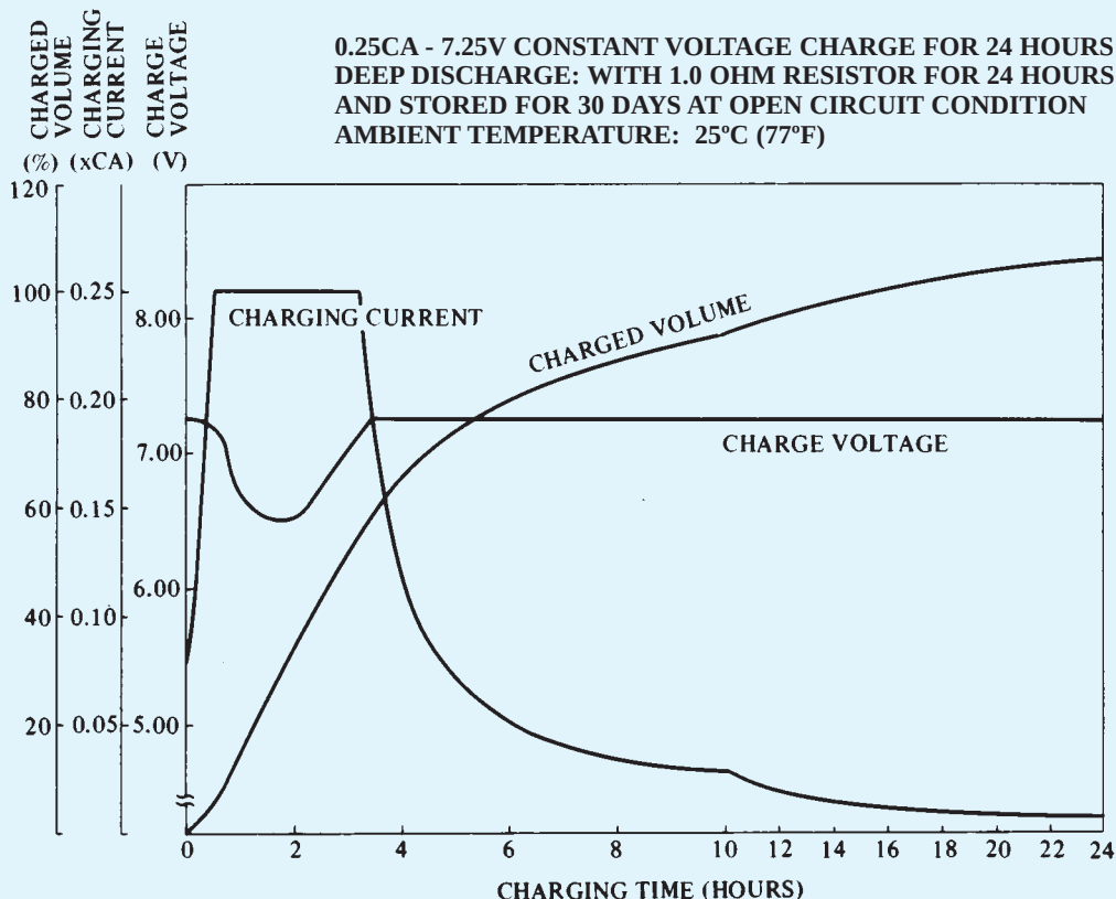
Figure 24. TYPICAL CHARGING CHARACTERISTICS AFTER DEEP DISCHARGE
