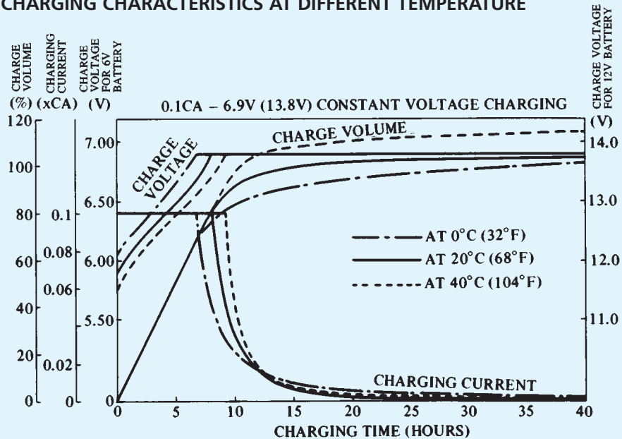
Figure 21. CHARGING CHARACTERISTICS AT DIFFERENT TEMPERATURE
