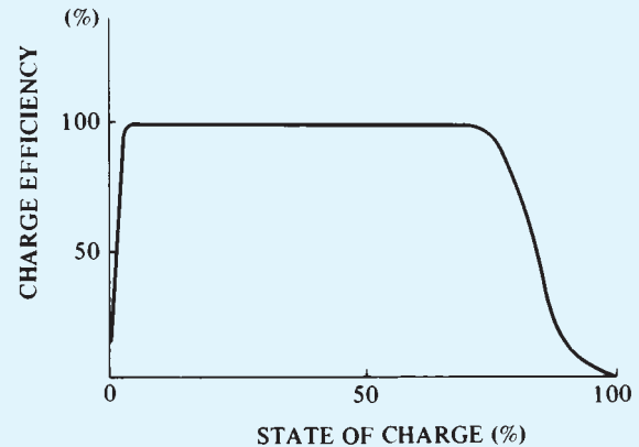
Figure 26. CHARGING EFFICIENCY VS STATE OF CHARGE
