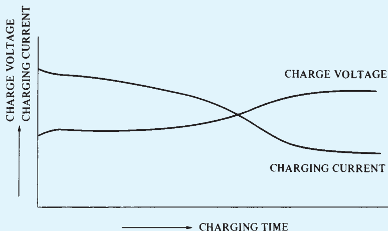
Figure 17. CHARGING CHARACTERISTICS OF A TAPER CHARGER
