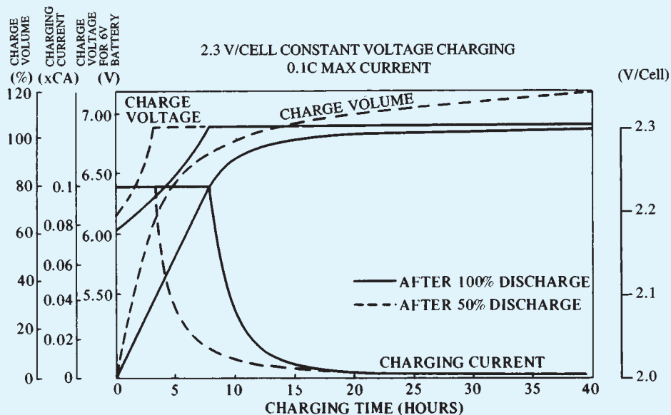
Figure 8. CHARGING CHARACTERISTICS
