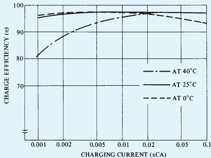
Figure 27. CHARGING EFFICIENCY
