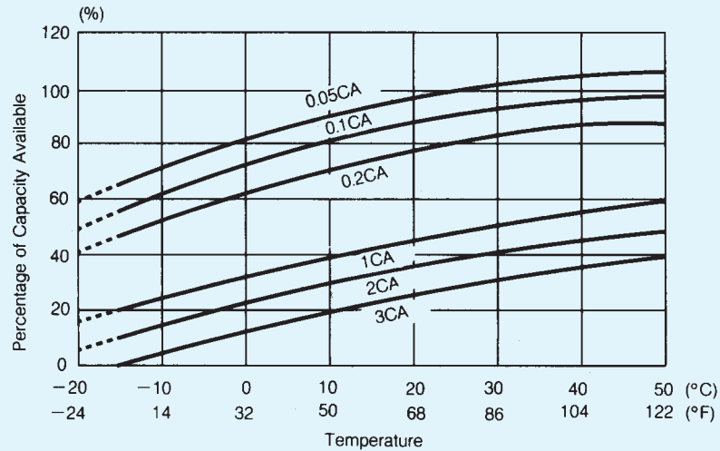
Figure 7. TEMPERATURE EFFECTS IN RELATION TO BATTERY CAPACITY
