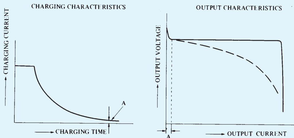
Figure 23. TAPER-CURRENT CHARGING CIRCUITS
