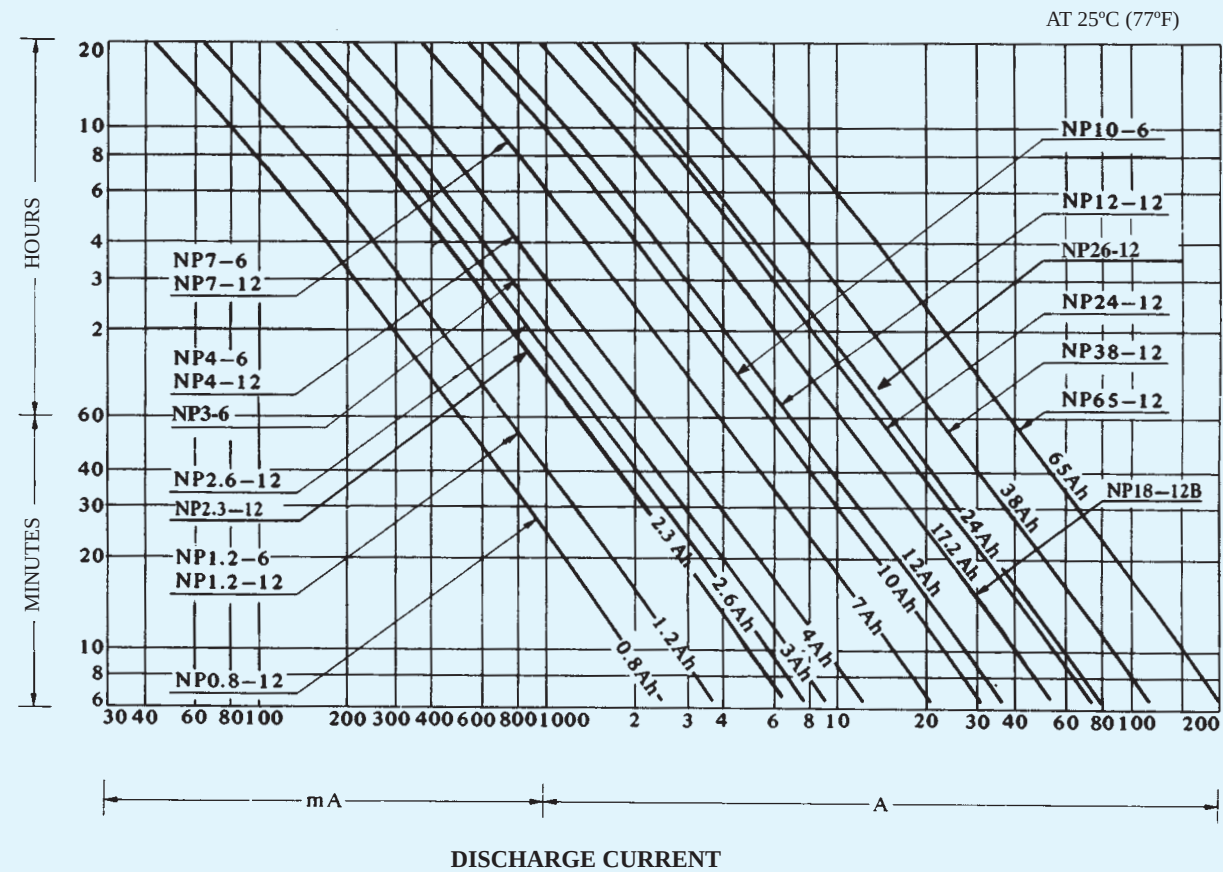
Figure 1. 20-HOUR RATE CAPACITY SELECTION CHART
