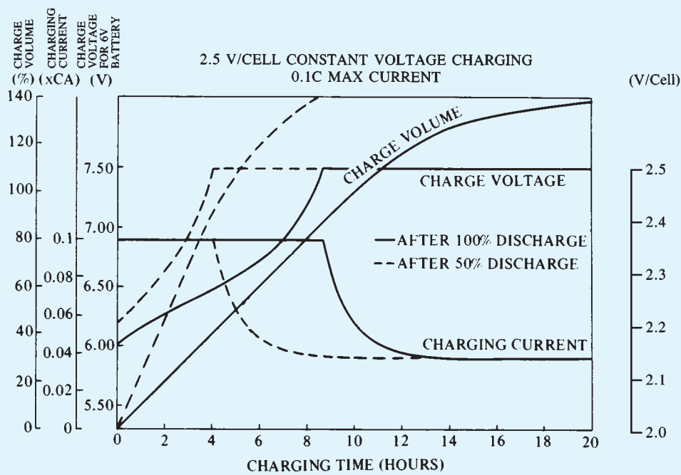
Figure 10. CHARGING CHARACTERISTICS
