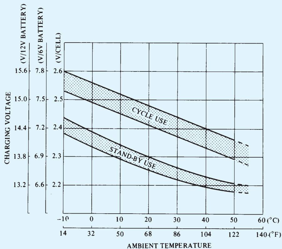
Figure 25. RELATIONSHIP BETWEEN CHARGING VOLTAGE AND TEMPERATURE
